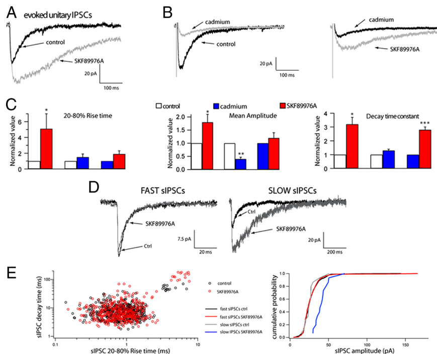
Figure 3. Kinetics of NGFC-IPSCs at low release probability and in the presence of a GAT-1 blocker. A, B , Representative traces of NGFC-IPSCs in control or in the presence of 10 \mu M CdCl 2 showing the effect of application of 25 \mu M SKF89976A (each trace is an average of 5 sweeps). C , Quantification of the effects of cadmium or SKF89976A on 20–80% rise time, amplitude, and decay time constant of the IPSCs. Note that SKF89976A is applied either alone (left red bars for each graph) or in the presence of Cd 2+ (right red bars for each graph). Any statistical difference is highlighted with asterisks (* p < 0.05 , ** p < 0.01 , *** p < 0.005 ; n = 5 for SKF89976A, n = 8 for Cd 2+ , n = 4 for Cd 2+ plus SKF89976A). Error bars indicate SEM. D , Representative examples of fast sIPSCs and slow sIPSCs recorded in NGFCs in control conditions and after application of 25 \mu M SKF89976A. E , Quantification of the effect of SKF89976A on sIPSCs. The left graph shows the analysis of 10–90% rise time (in milliseconds) versus decay time constant (in milliseconds) of 500 sIPSCs recorded from NGFCs ( n = 5 ). Note the appearance of two populations: a fast rising, fast decaying events (fast sIPSCs), and slowly rising (>3 ms), slowly decaying (>40 ms) events (slow sIPSCs). The two distributions were highly significantly different ( p < 0.001 , Kolmogorov–Smirnov test here and onward). The application of SKF89976A enhanced the rise time and the decay time constant of the slow sIPSCs ( p < 0.001 ) but not of the fast sIPSCs ( p > 0.1 ). In addition, SKF89976A enhanced the amplitude of the slow sIPSCs ( p < 0.001 ) but not of the fast sIPSCs ( p > 0.1 ). This latter action is shown in the cumulative plots (right) of the amplitude of fast sIPSCs (number of events, 485) and slow sIPSCs (number of events, 15) in control or during SKF89976A as indicated.
