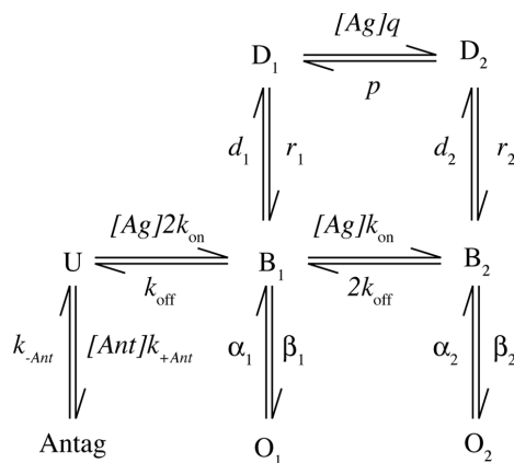
Supplemental Figure 6. The Kinetic model used to simulate GABA A receptors underlying phasic slow IPSCs, and to estimate the profile of GABA exposure. The model contains an unbound state (U), two transient agonist bound states (B 1 , B 2 ), two open states (O 1 , O 2 ), two desensitized states (D 1 , D 2 ) and one competitive antagonist-bound state (Antag). Agonist and antagonist concentrations ([Ag], [Ant]) scale the binding transitions. The two agonist binding sites are assumed to be equal and independent for simplicity.
