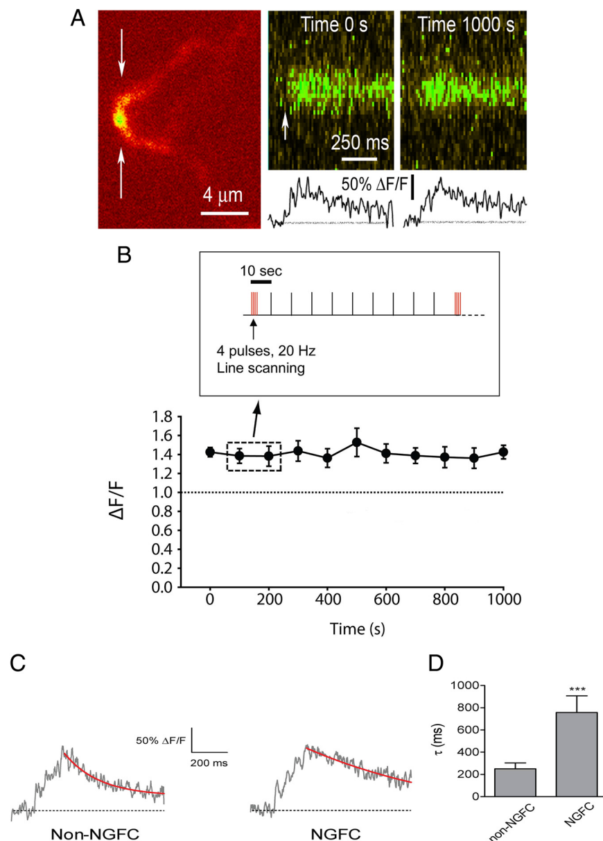
Figure 9. Changes in presynaptic Ca 2+ signal do not contribute to the synaptic depression. A , Image of an axonal varicosity of a NGFC (left panel) and Ca 2+ transients at the beginning (time 0 s) and at the end (time 1000 s) of the protocol shown in B . The morphological tracer Alexa Fluor 594 (40 μM) and the Ca 2+ indicator Fluo-4 (200 μM) were used. The protocol consisted of intracellular stimulation with four action potentials at 20 Hz every 10 s for ~17 min. B , The Ca 2+ transients detected in axonal boutons of NGFCs by this protocol were stable and no significant changes were observed during 1000 s of stimulation. The plot shows average values ± SEM ( n = 8 ). C , Fluorescence transients from non-NGFC (left) and NGFC boutons (right) induced by trains of four somatic pulses applied through the whole-cell electrode. Each transient is an average of at least 10 trials. Monoexponential functions were fitted to the decay phase of the transient just after the last pulse of the trains. D , Summary of the data for the decay time constant of the fluorescence transients for both types of cells. The Ca 2+ signals from NGFCs decay three times slower than in other types of interneurons (data are mean ± SEM from NGFCs or other interneurons with the soma in the SLM; n = 6 each; *** p < 0.001 ).
